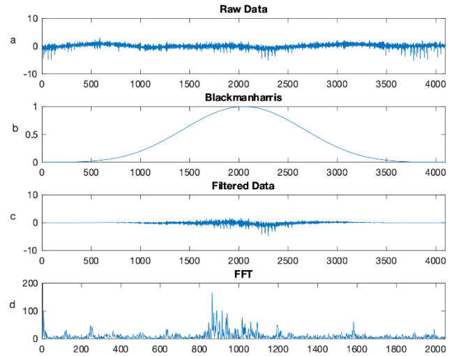
Figure 4. Acoustic chemometrics signal processing steps
